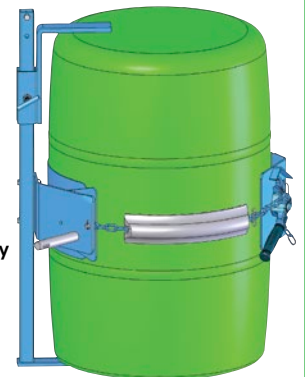
DC279 Bracket Assembly
